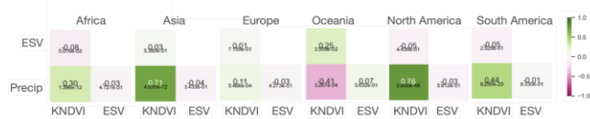
Figure 2. Pearson correlation and p-values between scaled ESV, precipitation, and kNDVI per continent.
